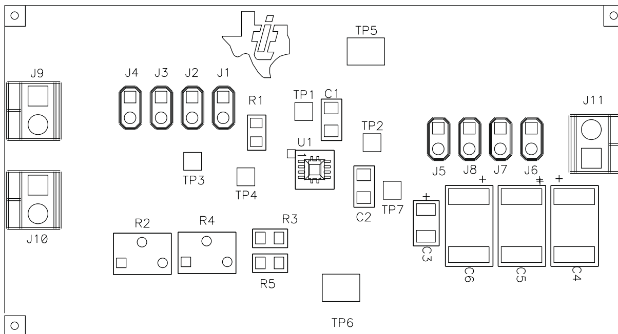
Figure 3. Top-Side Layout
