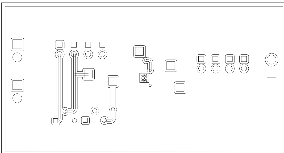
Figure 4. Bottom-Side Layout
